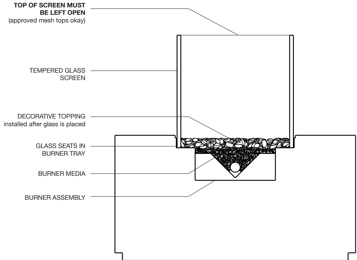
SECTION DIAGRAM
