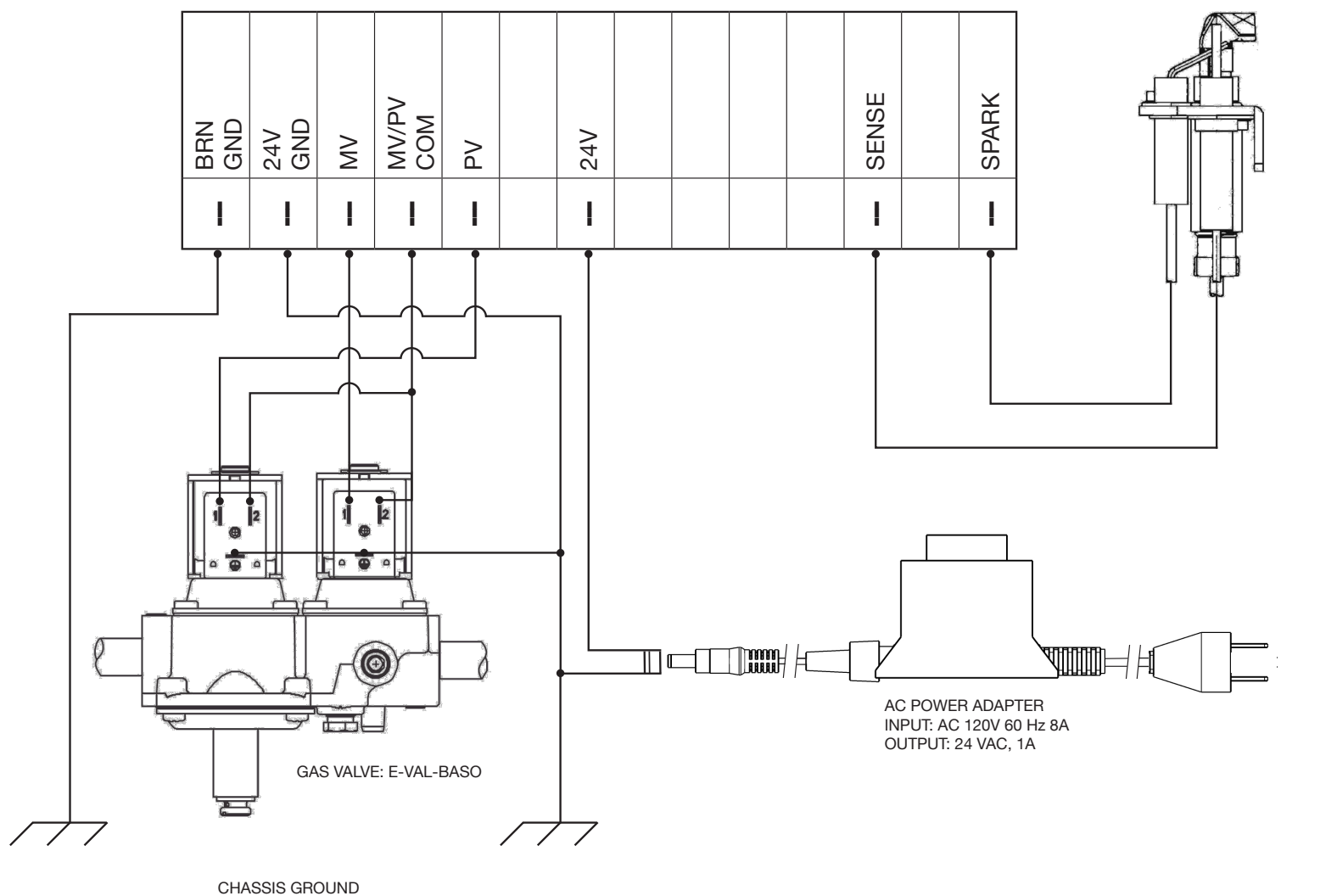
IGNITION CONTROL BOARD - BASO C-SERIES
