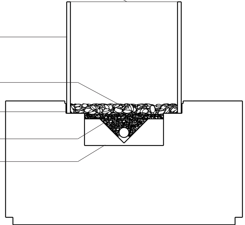
SECTION DIAGRAM
