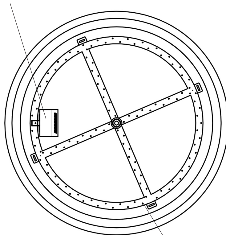
PILOT ASSEMBLY
